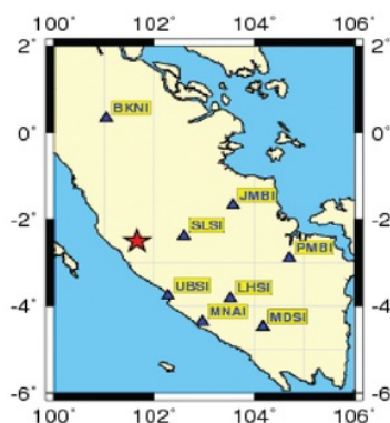
Fig. 2. Earthquake occurred in south Sumatera province on July 13, 2010 with the epicenter indicated by red star and distribution of the eight seismic stations as blue triangles providing the three-components of seismic broadband-noises used in this research.
