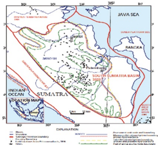
Figure 1. Index map of South Sumatra Basin Province, 2010. This map locates the epicenter of active source rock and one Total Petroleum System, Late Tertiary Akar-Cenozoic (SIS/BSI) with core assessment unit, South Sumatra (SIS/BSI).
