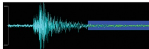
Fig. 4. The Z-component of broadband-noises (indicated by highlight blue) as recorded by JMBI seismic station after the quake occurred in south Sumatera province on July 13, 2010.
